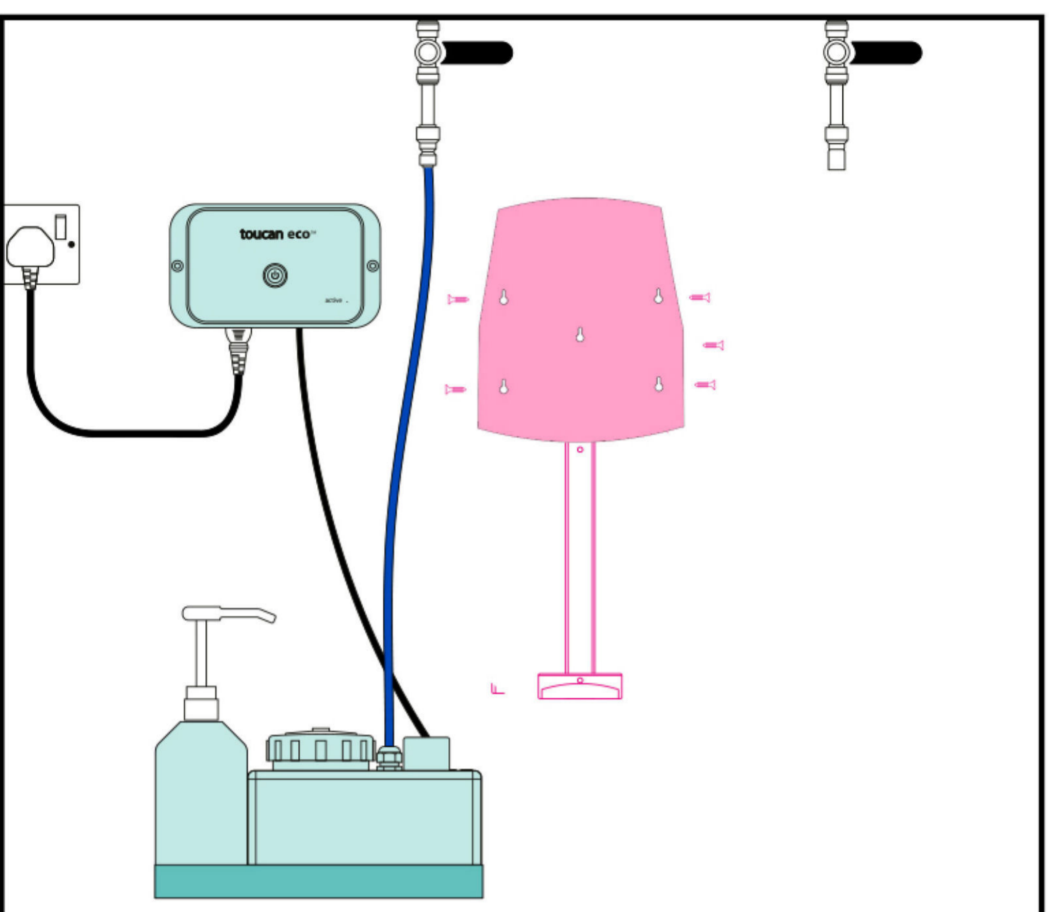
5l holding tank and control box.
